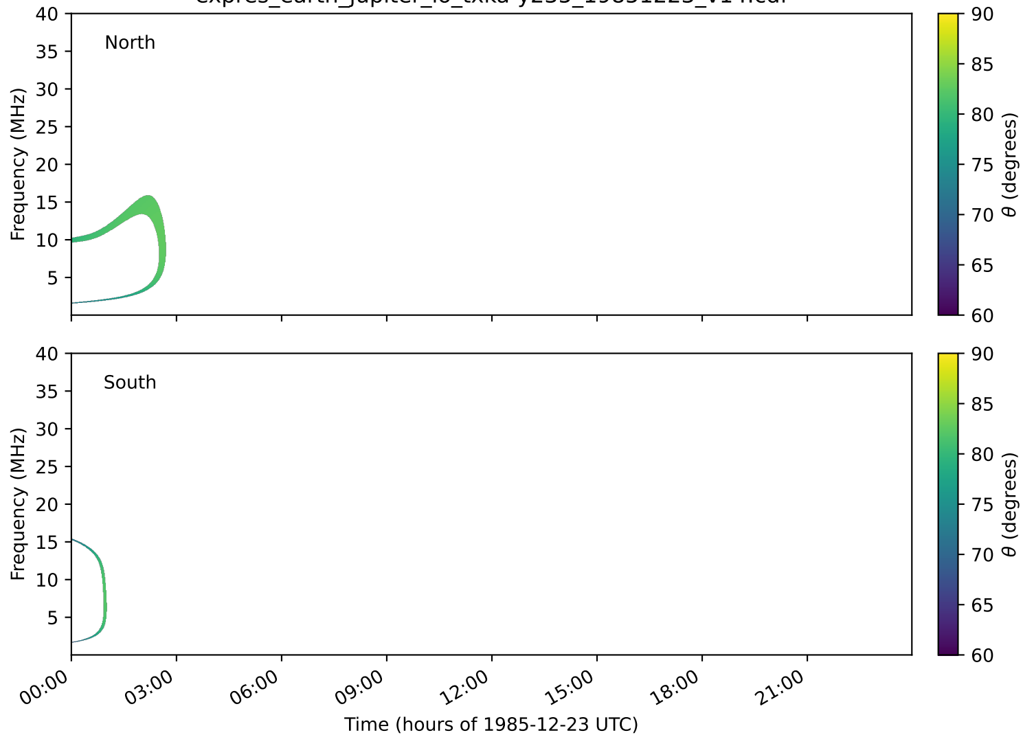
expres_earth_jupiter_io_txka-y235_19851223_v14.cdf
