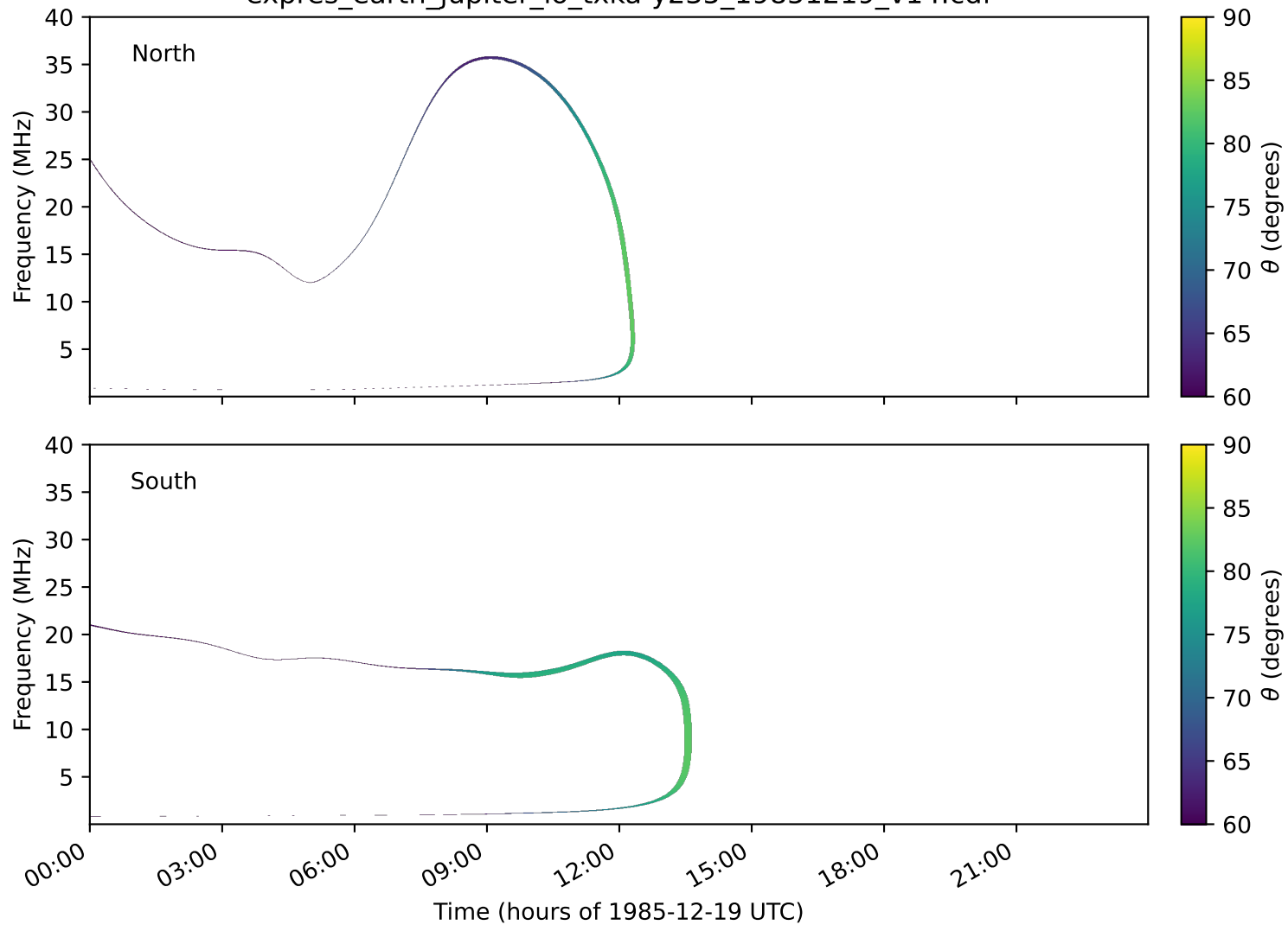
expres_earth_jupiter_io_txka-y235_19851219_v14.cdf
