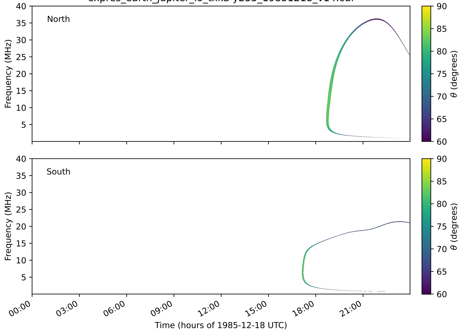
expres_earth_jupiter_io_txka-y235_19851218_v14.cdf
