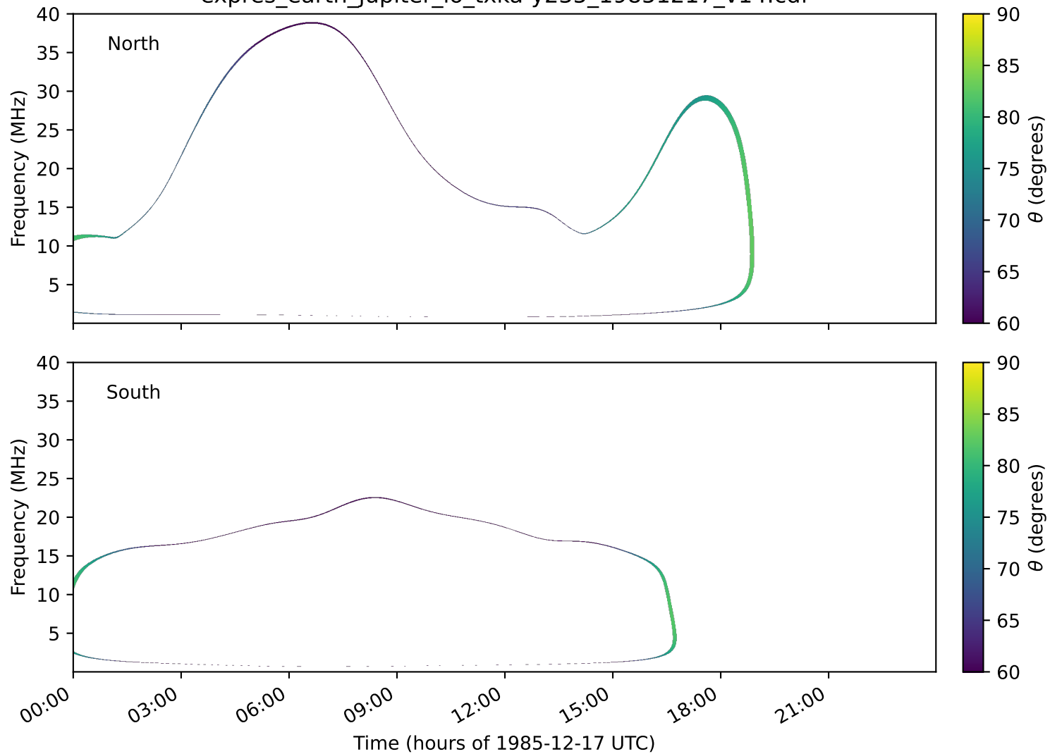
expres_earth_jupiter_io_txka-y235_19851217_v14.cdf
