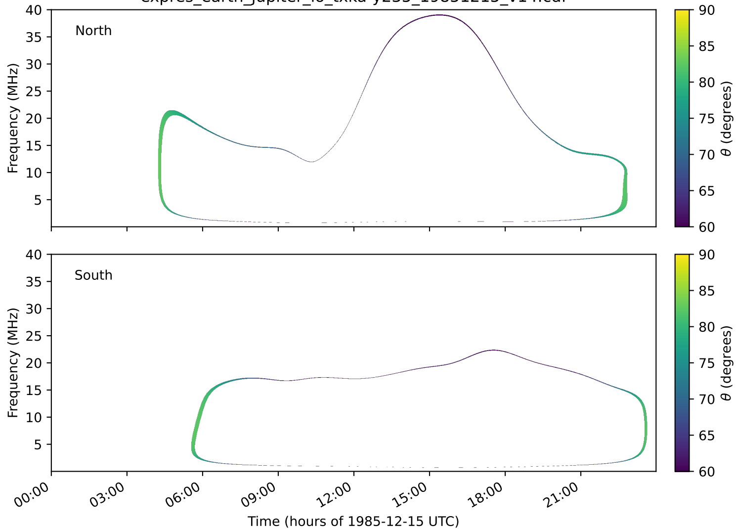
expres_earth_jupiter_io_txka-y235_19851215_v14.cdf
