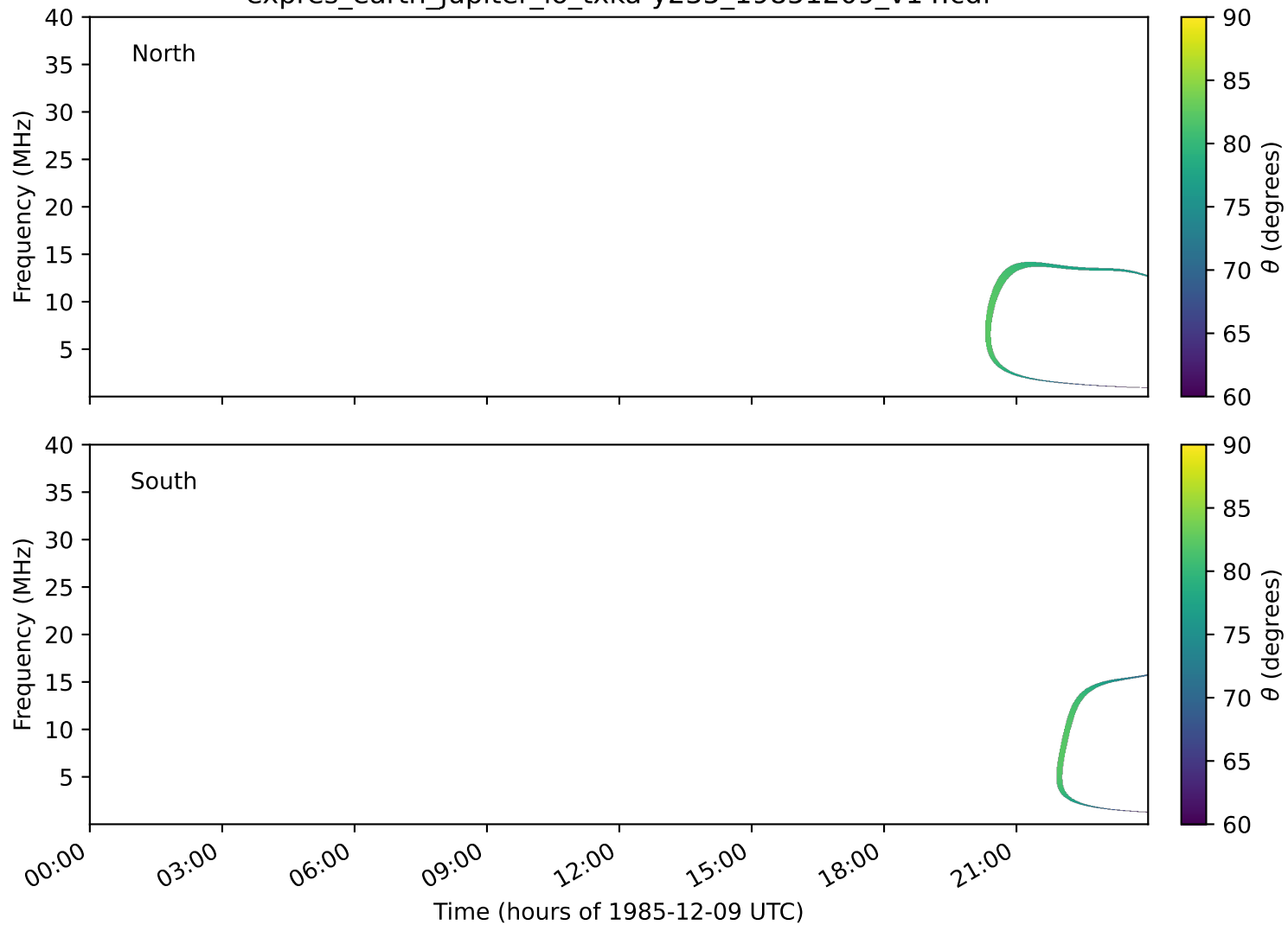
expres_earth_jupiter_io_txka-y235_19851209_v14.cdf
