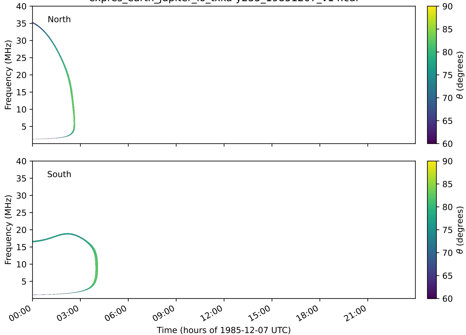
expres_earth_jupiter_io_txka-y235_19851207_v14.cdf
