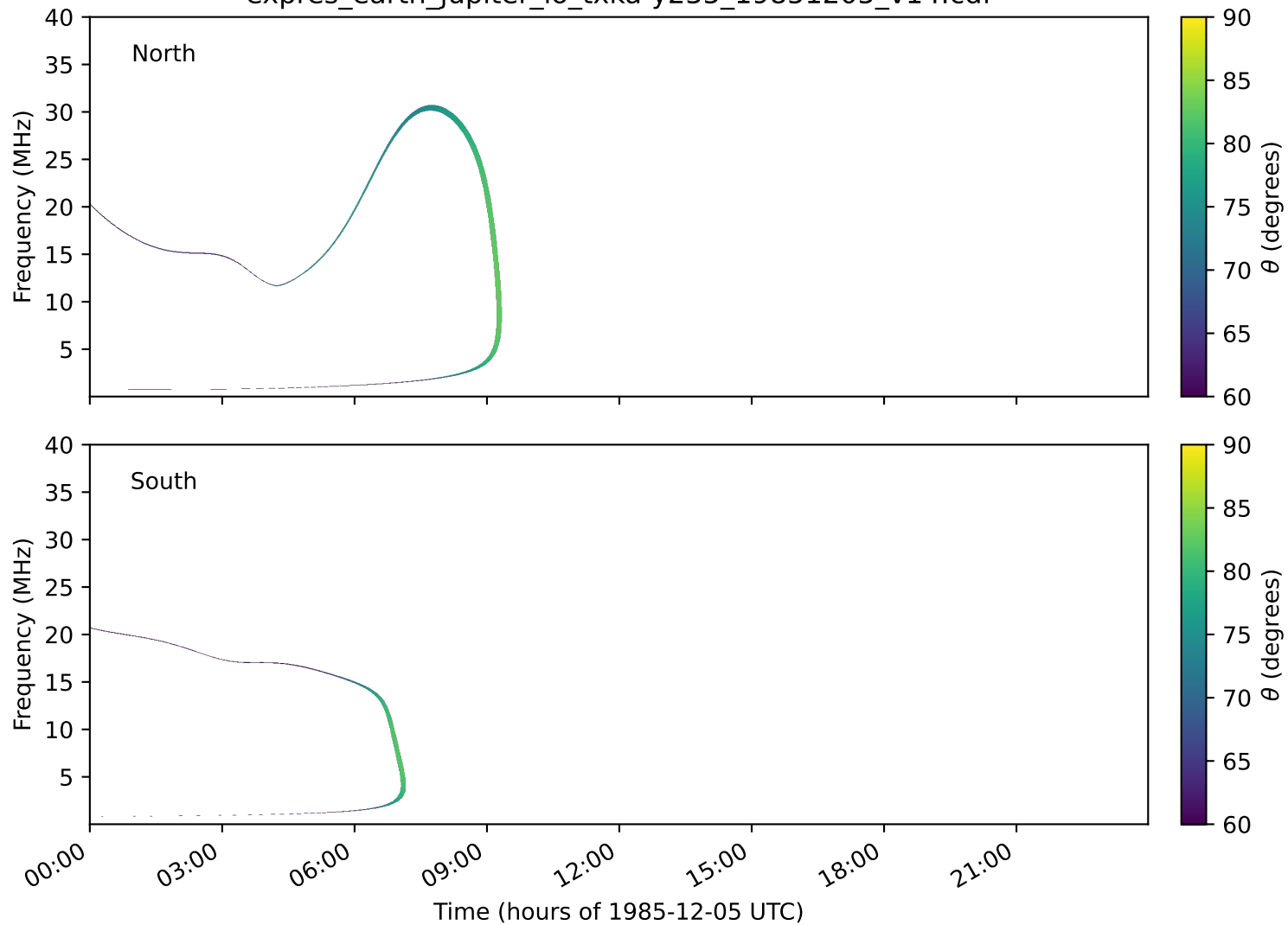
expres_earth_jupiter_io_txka-y235_19851205_v14.cdf
