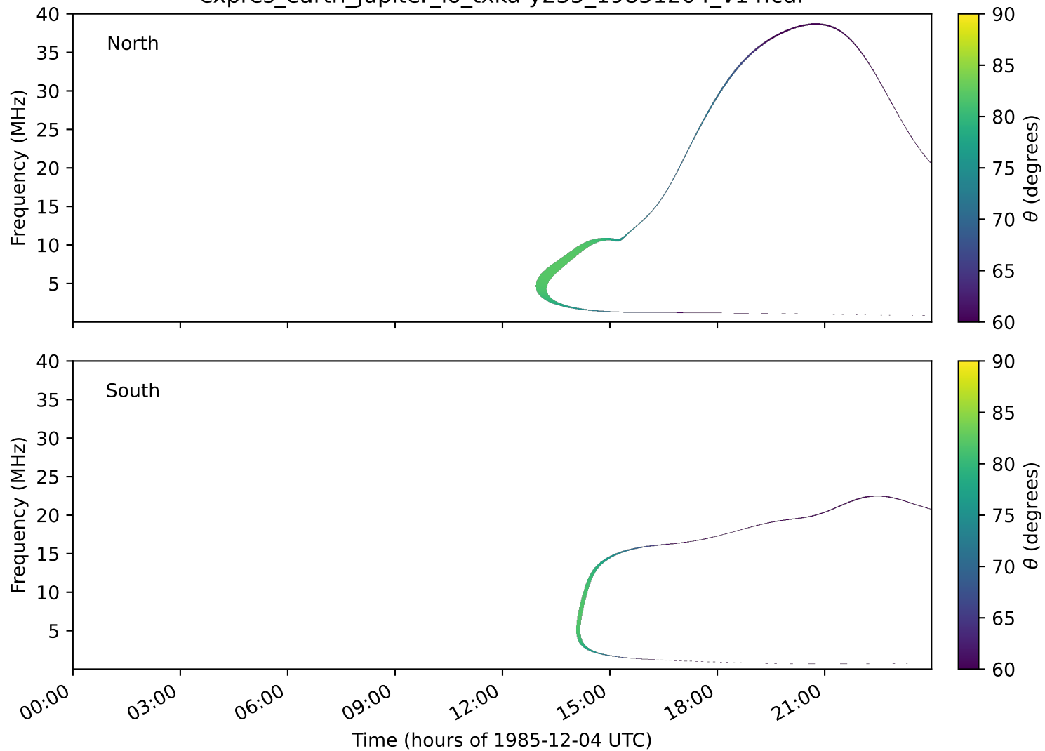
expres_earth_jupiter_io_txka-y235_19851204_v14.cdf
