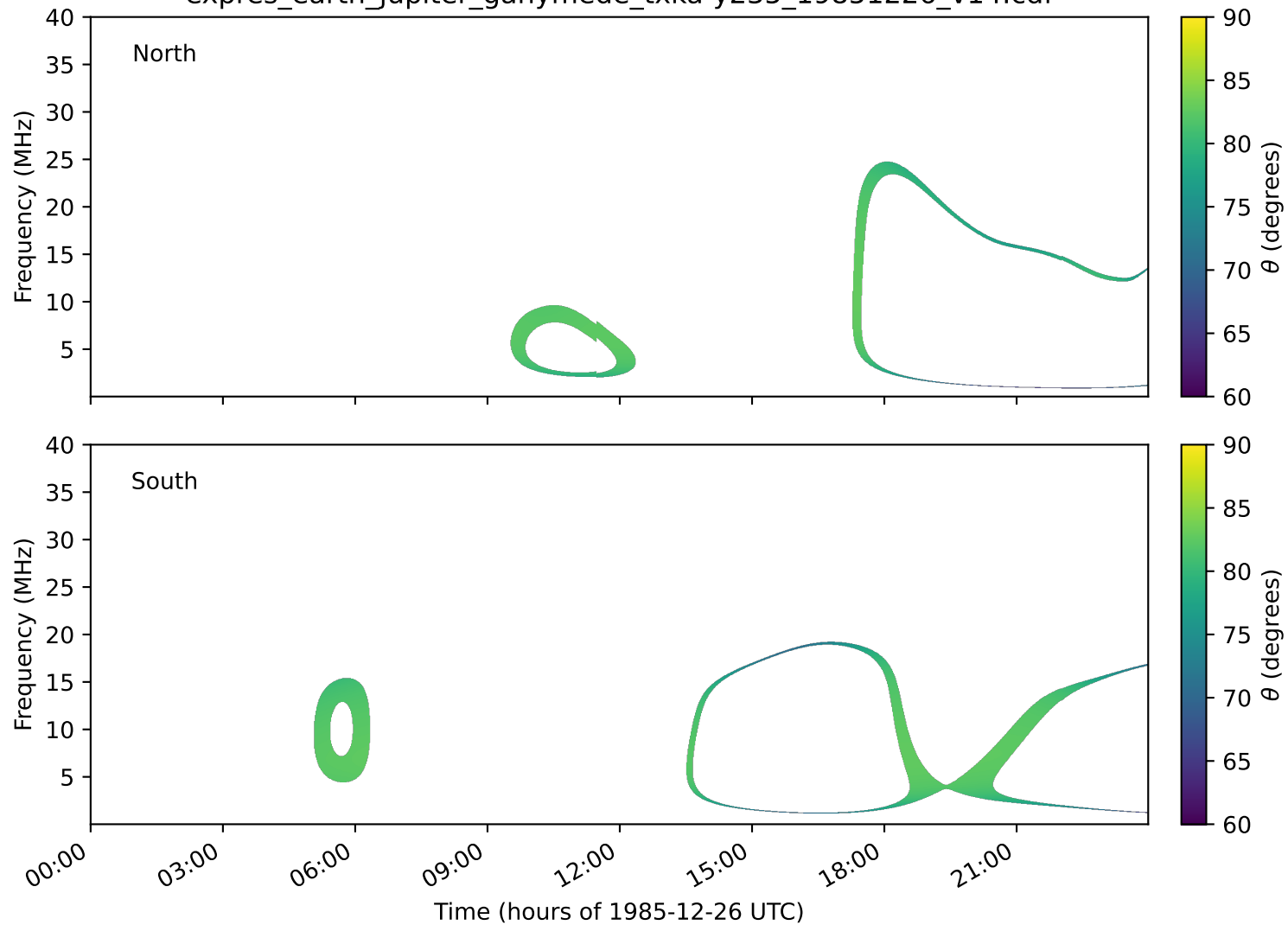
expres_earth_jupiter_ganymede_txka-y235_19851226_v14.cdf
