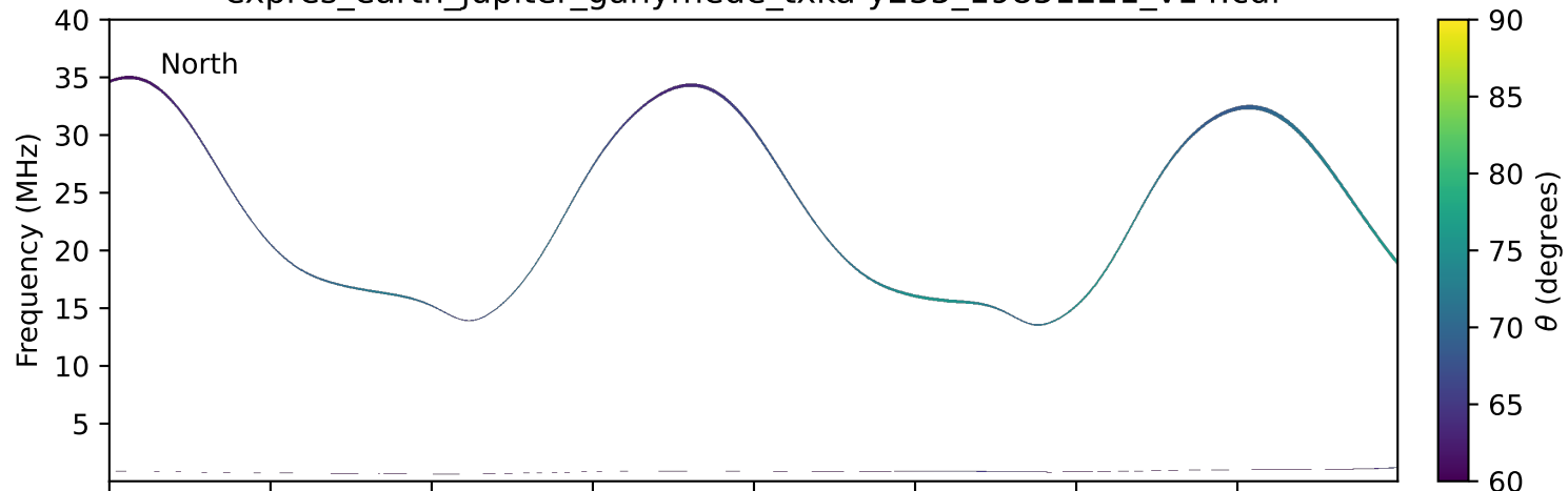
expres_earth_jupiter_ganymede_txka-y235_19851221_v14.cdf
