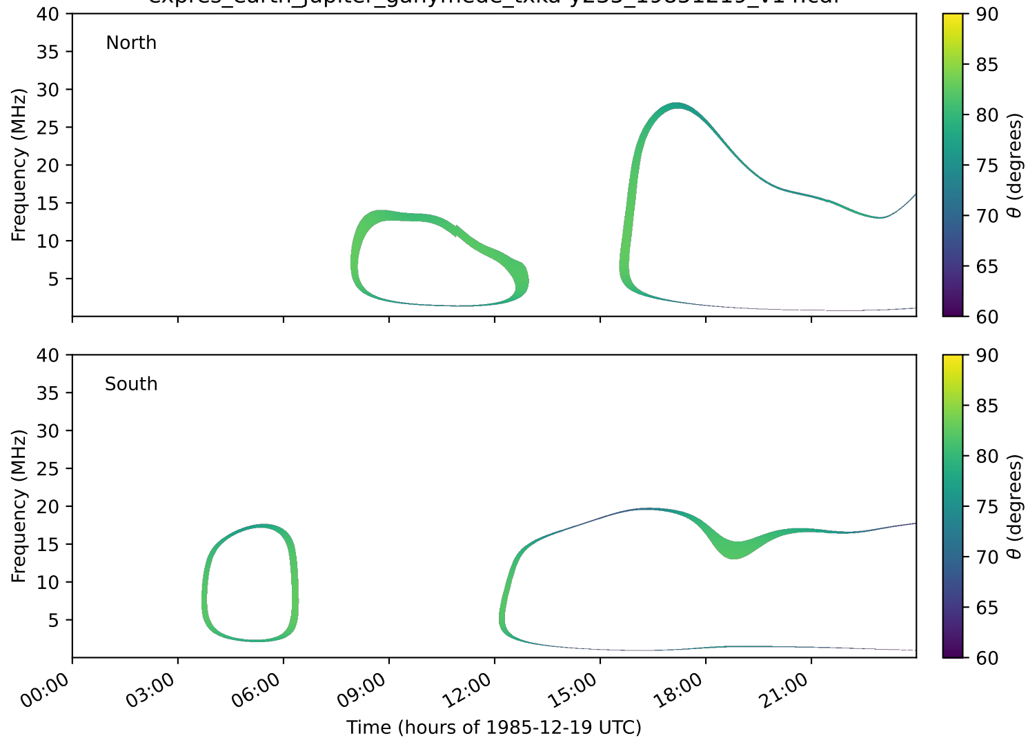
expres_earth_jupiter_ganymede_txka-y235_19851219_v14.cdf
