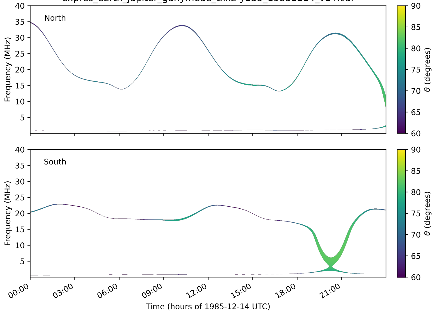
expres_earth_jupiter_ganymede_txka-y235_19851214_v14.cdf
