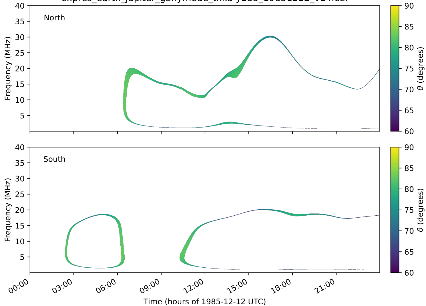
expres_earth_jupiter_ganymede_txka-y235_19851212_v14.cdf
