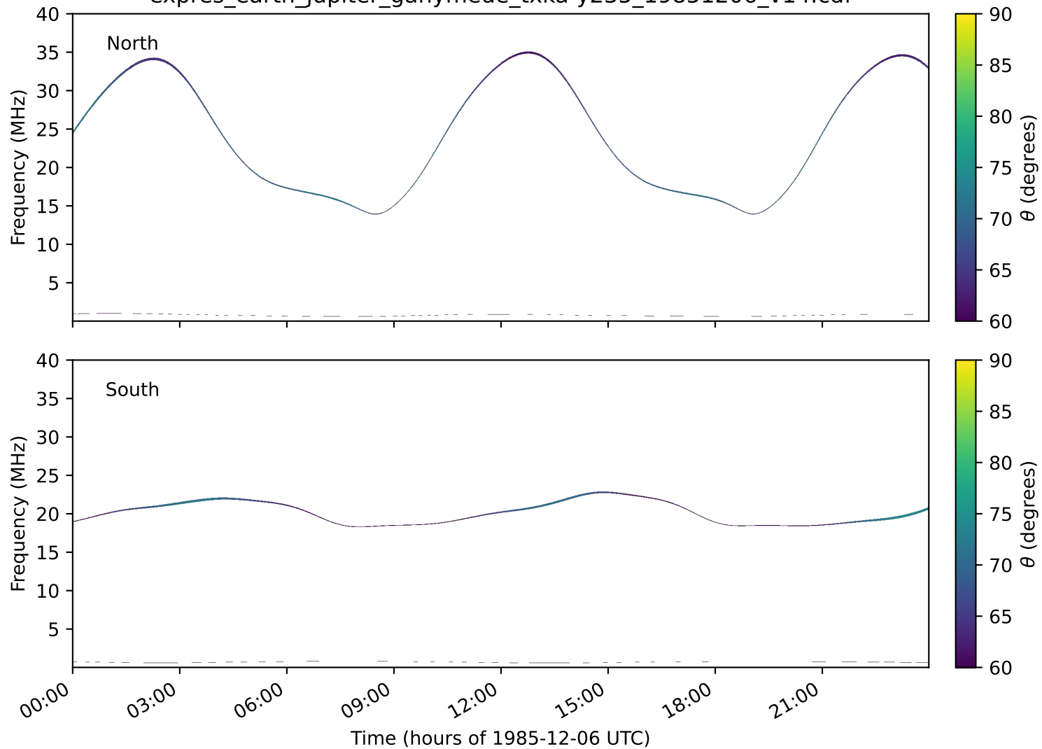
expres_earth_jupiter_ganymede_txka-y235_19851206_v14.cdf
