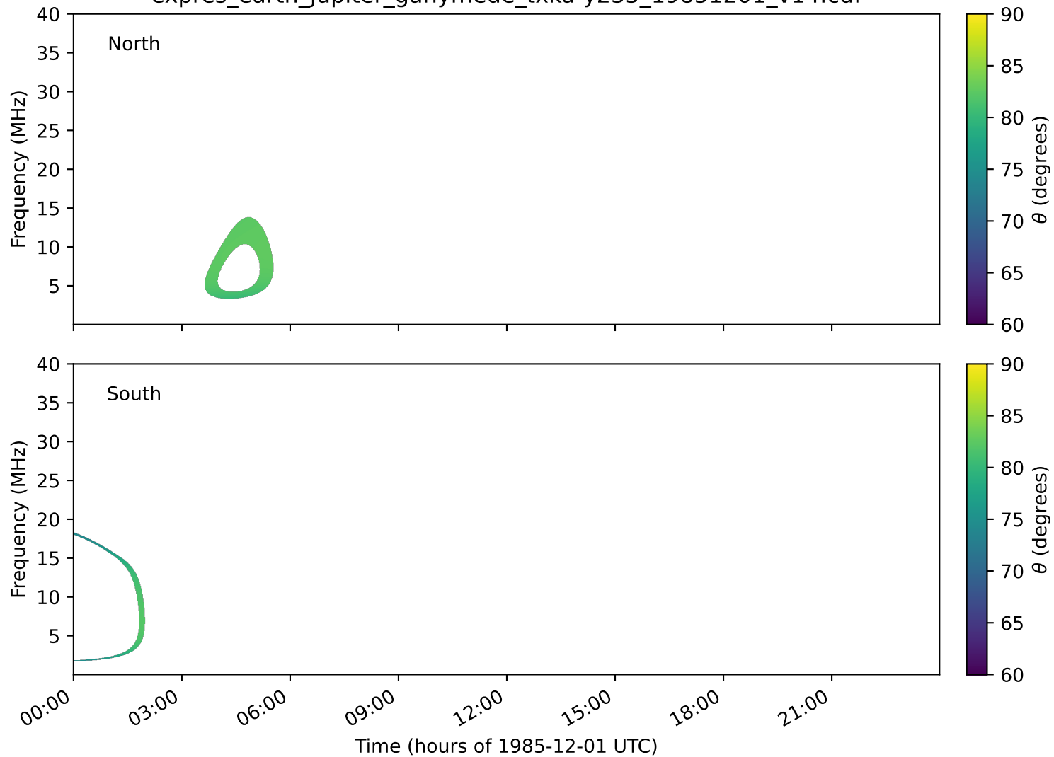
expres_earth_jupiter_ganymede_txka-y235_19851201_v14.cdf
