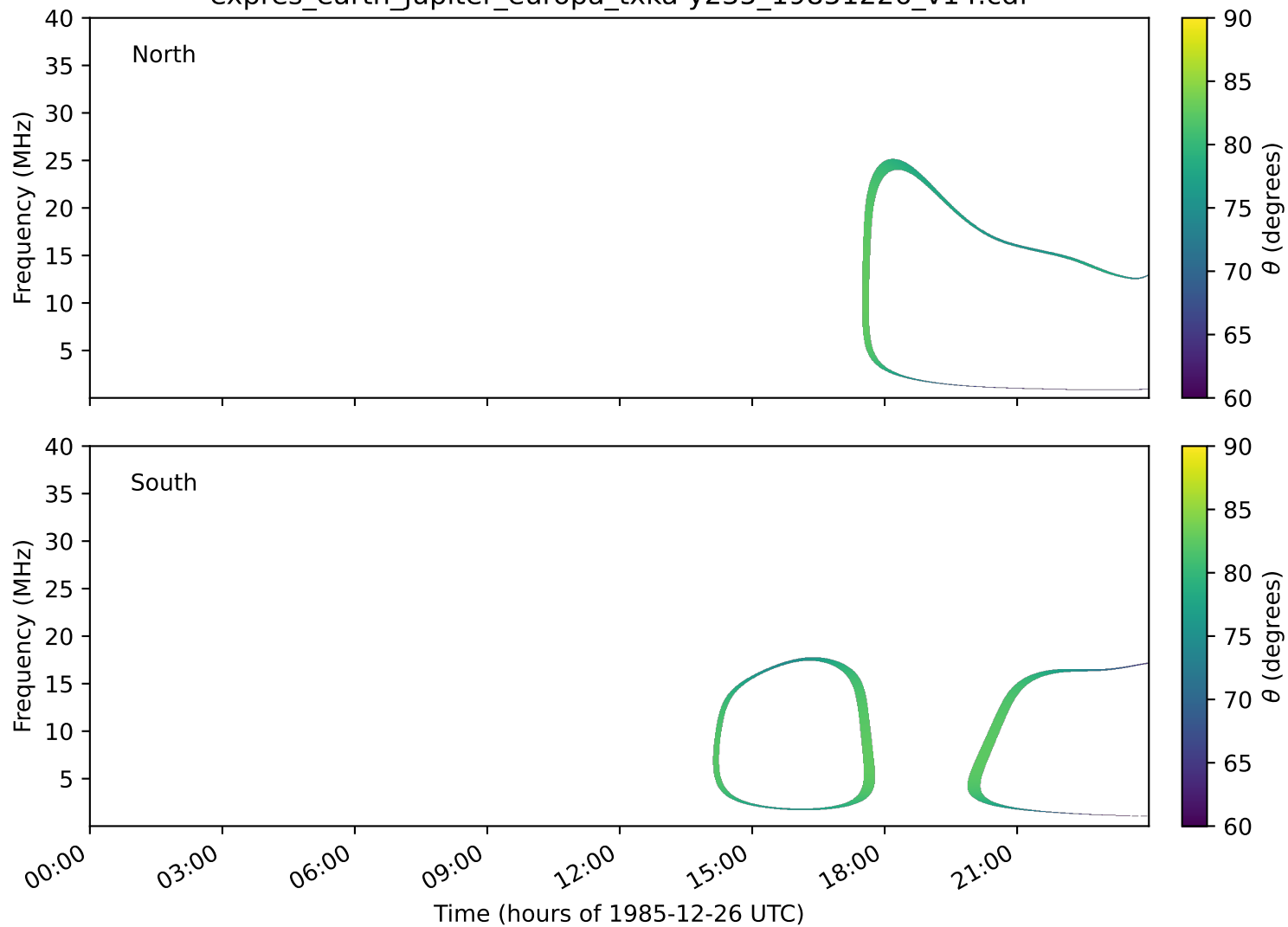
expres_earth_jupiter_europa_txka-y235_19851226_v14.cdf
