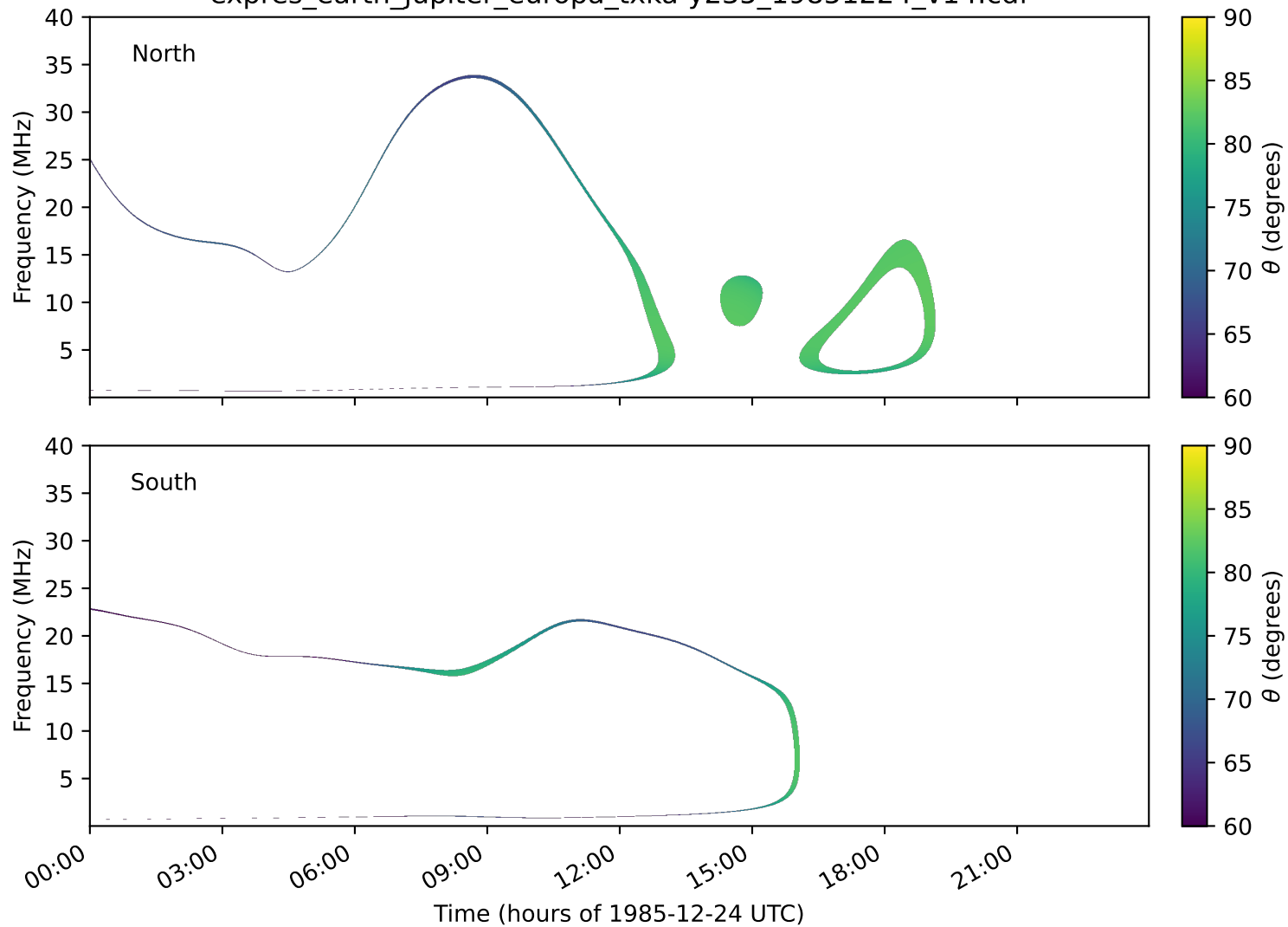
expres_earth_jupiter_europa_txka-y235_19851224_v14.cdf
