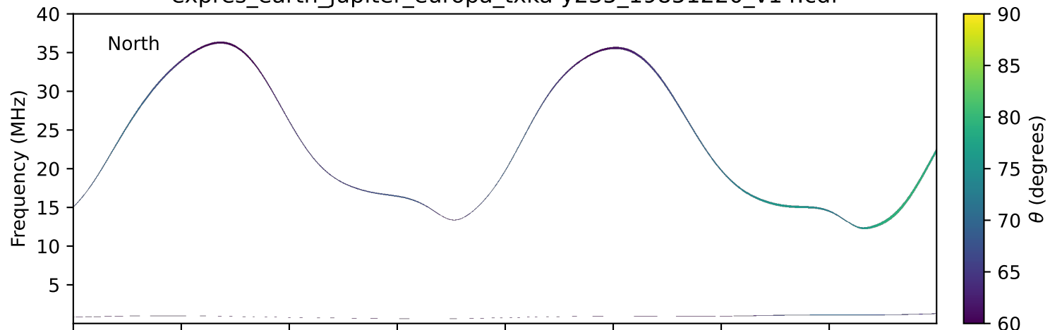
expres_earth_jupiter_europa_txka-y235_19851220_v14.cdf
