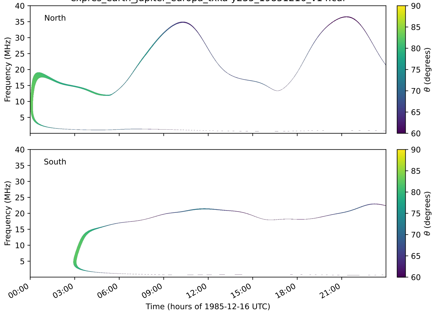
expres_earth_jupiter_europa_txka-y235_19851216_v14.cdf
