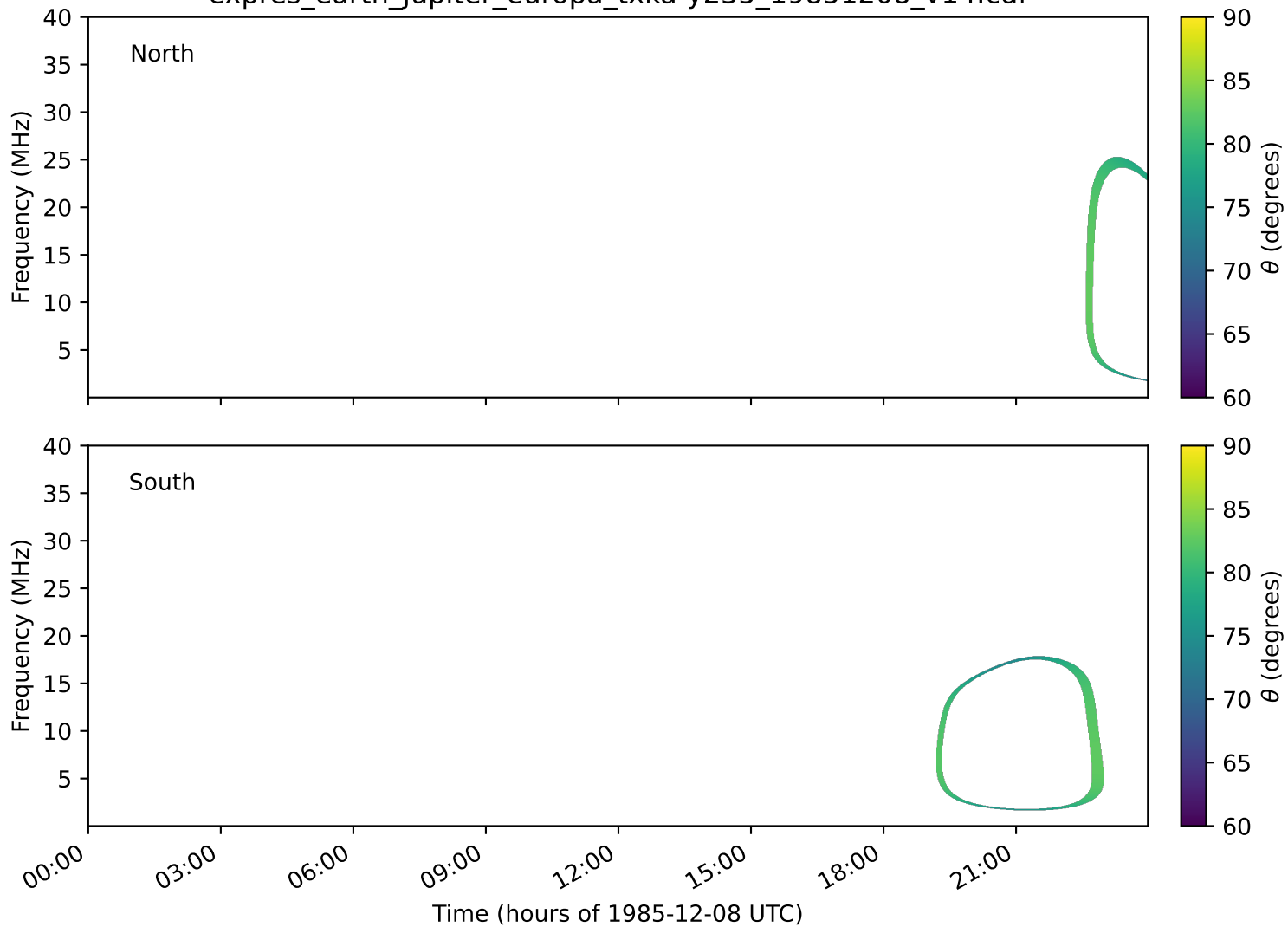
expres_earth_jupiter_europa_txka-y235_19851208_v14.cdf
