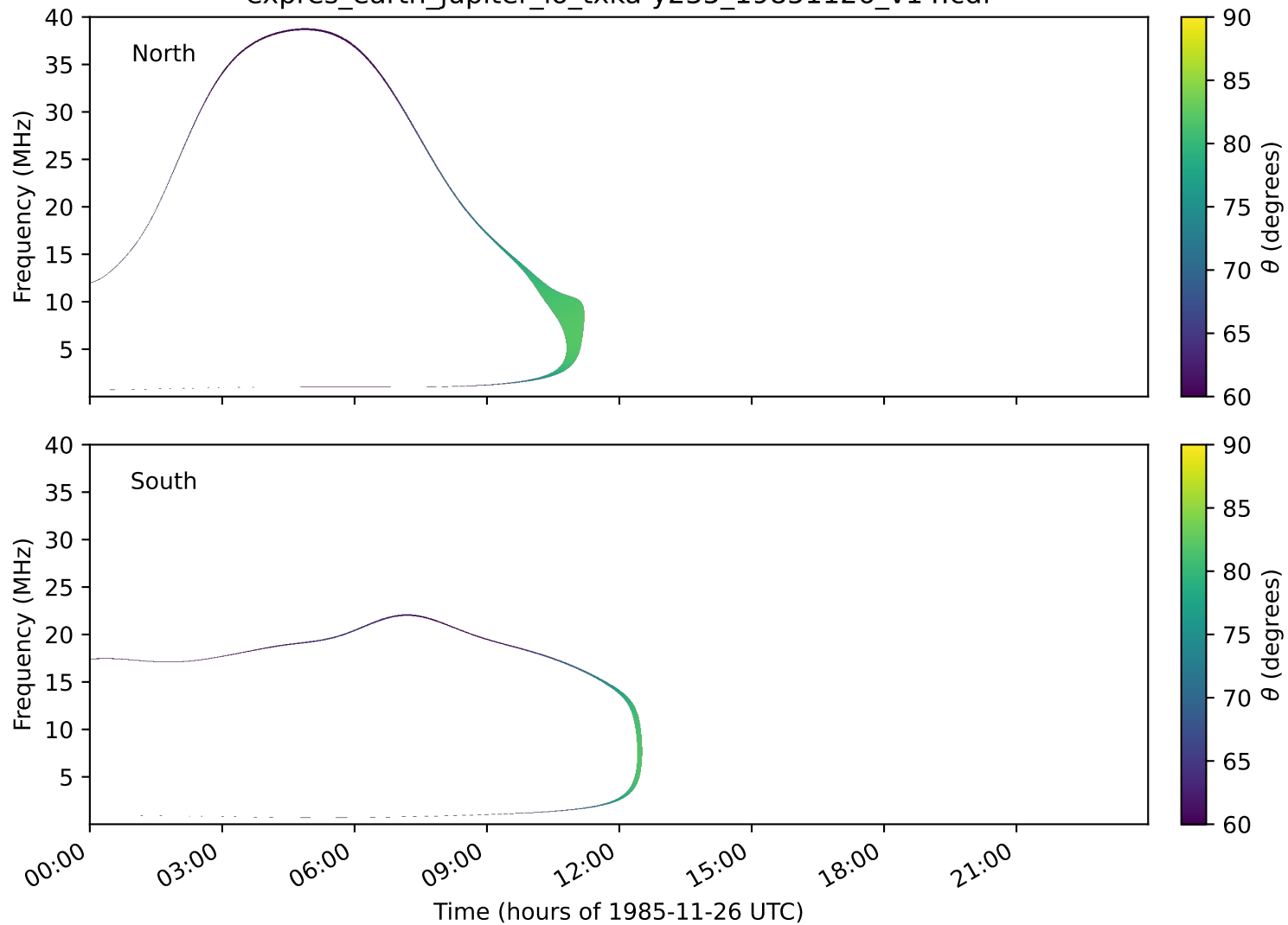
expres_earth_jupiter_io_txka-y235_19851126_v14.cdf
