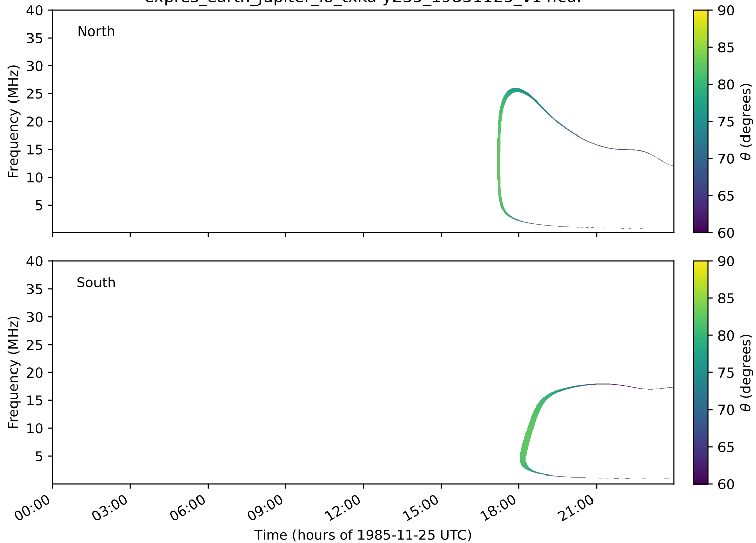
expres_earth_jupiter_io_txka-y235_19851125_v14.cdf
