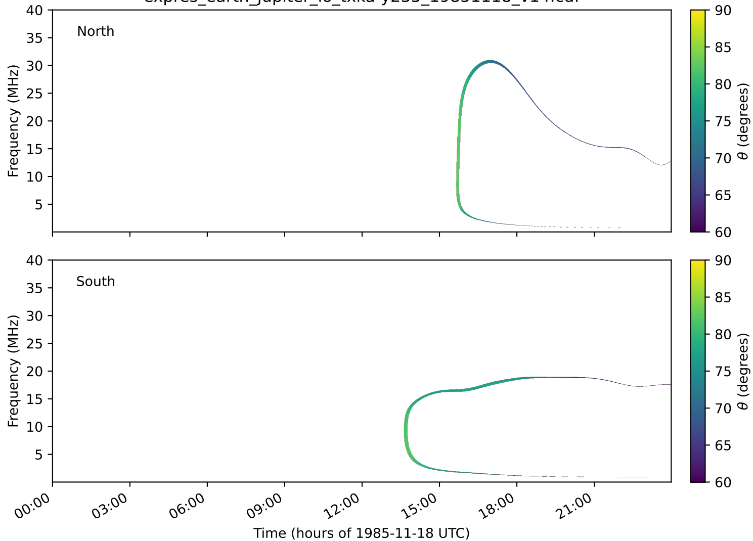
expres_earth_jupiter_io_txka-y235_19851118_v14.cdf
