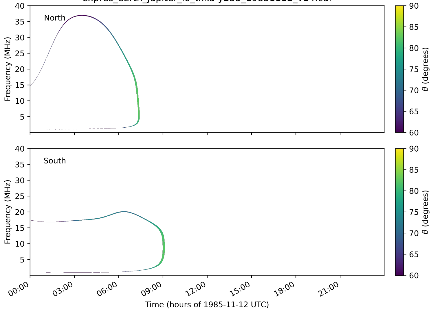
expres_earth_jupiter_io_txka-y235_19851112_v14.cdf
