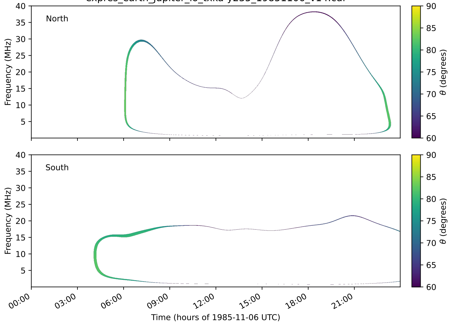
expres_earth_jupiter_io_txka-y235_19851106_v14.cdf
