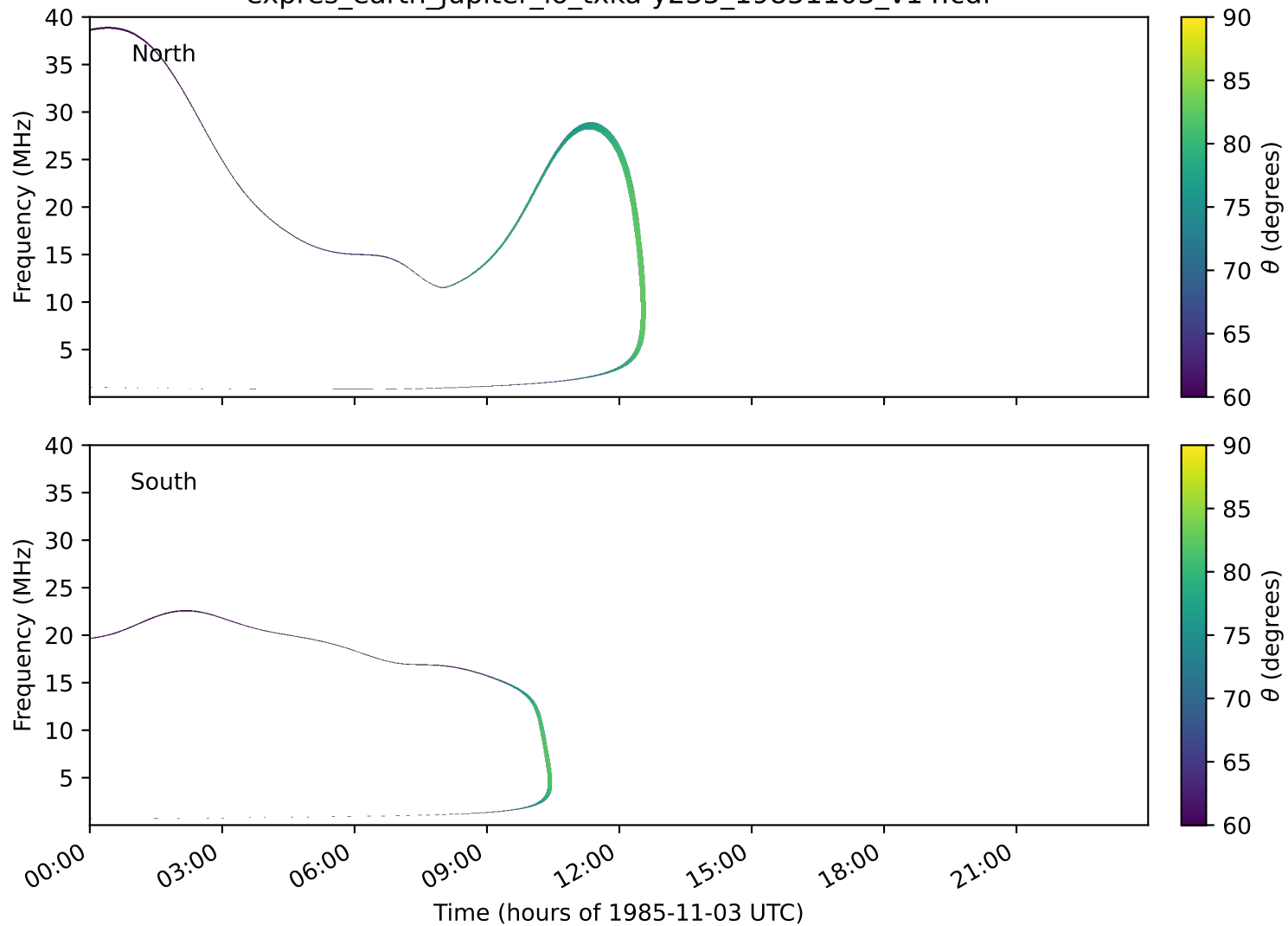
expres_earth_jupiter_io_txka-y235_19851103_v14.cdf
