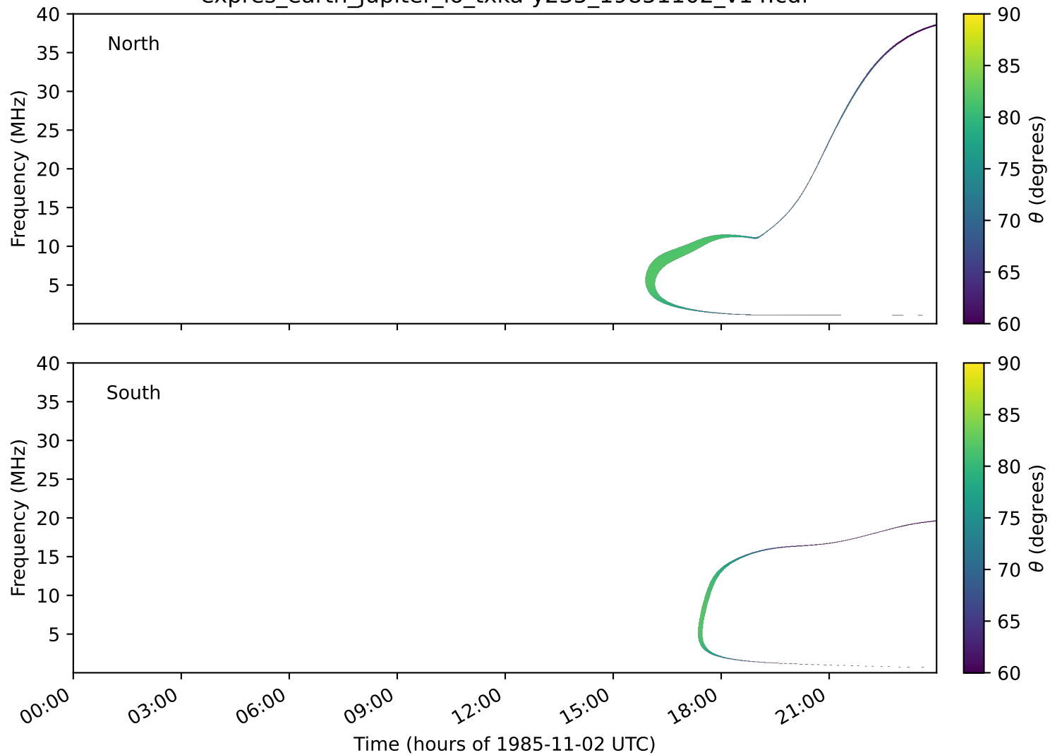
expres_earth_jupiter_io_txka-y235_19851102_v14.cdf
