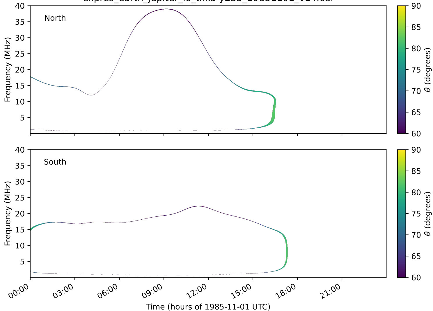
expres_earth_jupiter_io_txka-y235_19851101_v14.cdf
