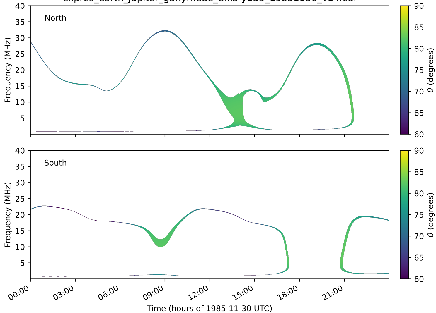
expres_earth_jupiter_ganymede_txka-y235_19851130_v14.cdf
