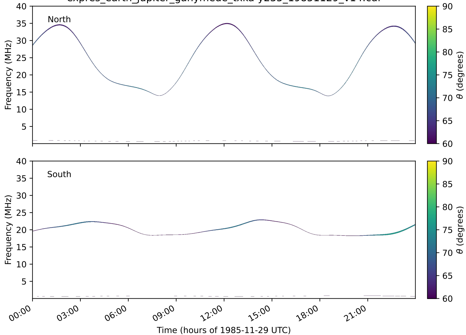
expres_earth_jupiter_ganymede_txka-y235_19851129_v14.cdf
