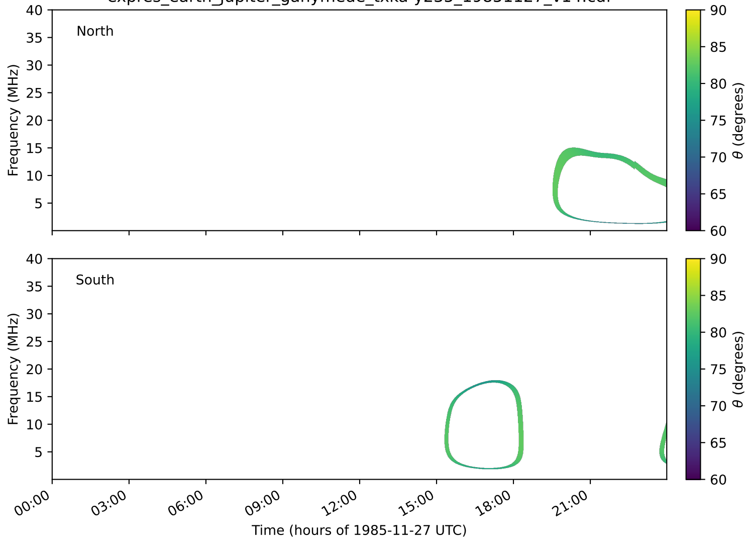
expres_earth_jupiter_ganymede_txka-y235_19851127_v14.cdf
