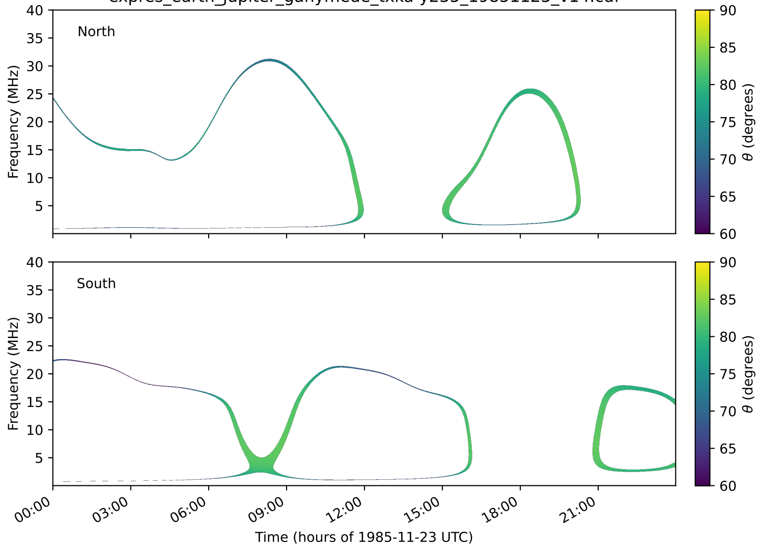
expres_earth_jupiter_ganymede_txka-y235_19851123_v14.cdf
