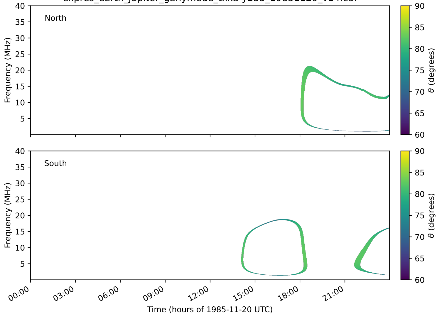
expres_earth_jupiter_ganymede_txka-y235_19851120_v14.cdf
