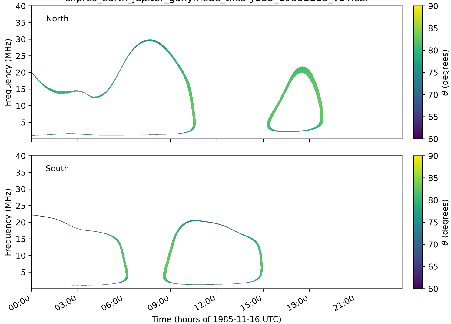
expres_earth_jupiter_ganymede_txka-y235_19851116_v14.cdf
