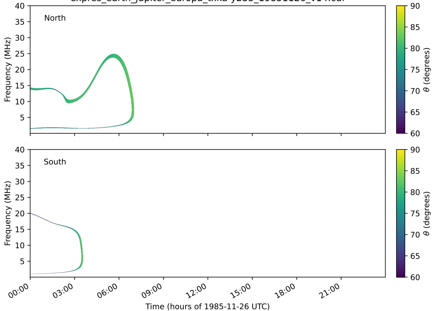
expres_earth_jupiter_europa_txka-y235_19851126_v14.cdf
