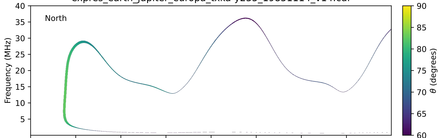
expres_earth_jupiter_europa_txka-y235_19851114_v14.cdf
