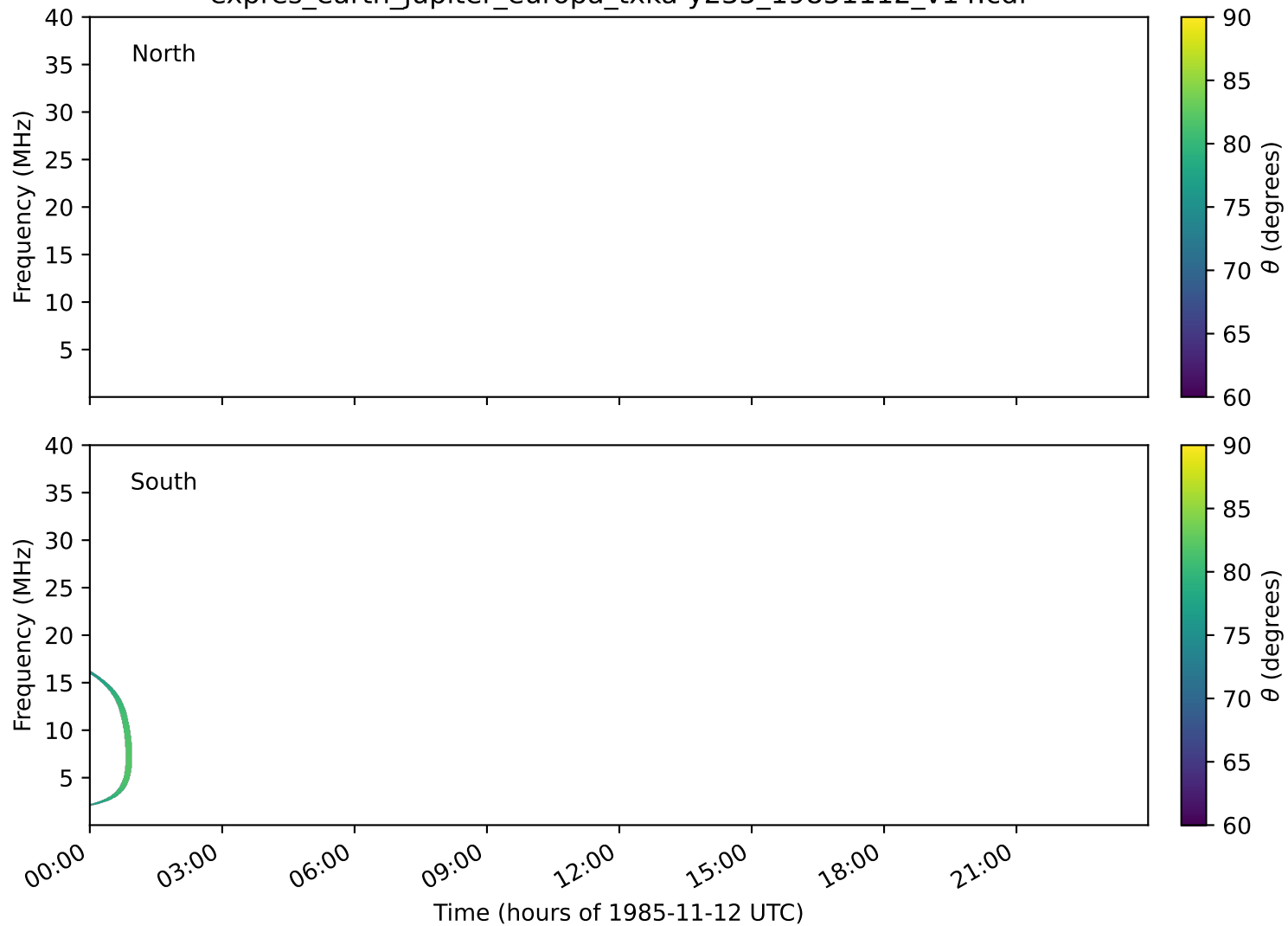
expres_earth_jupiter_europa_txka-y235_19851112_v14.cdf
