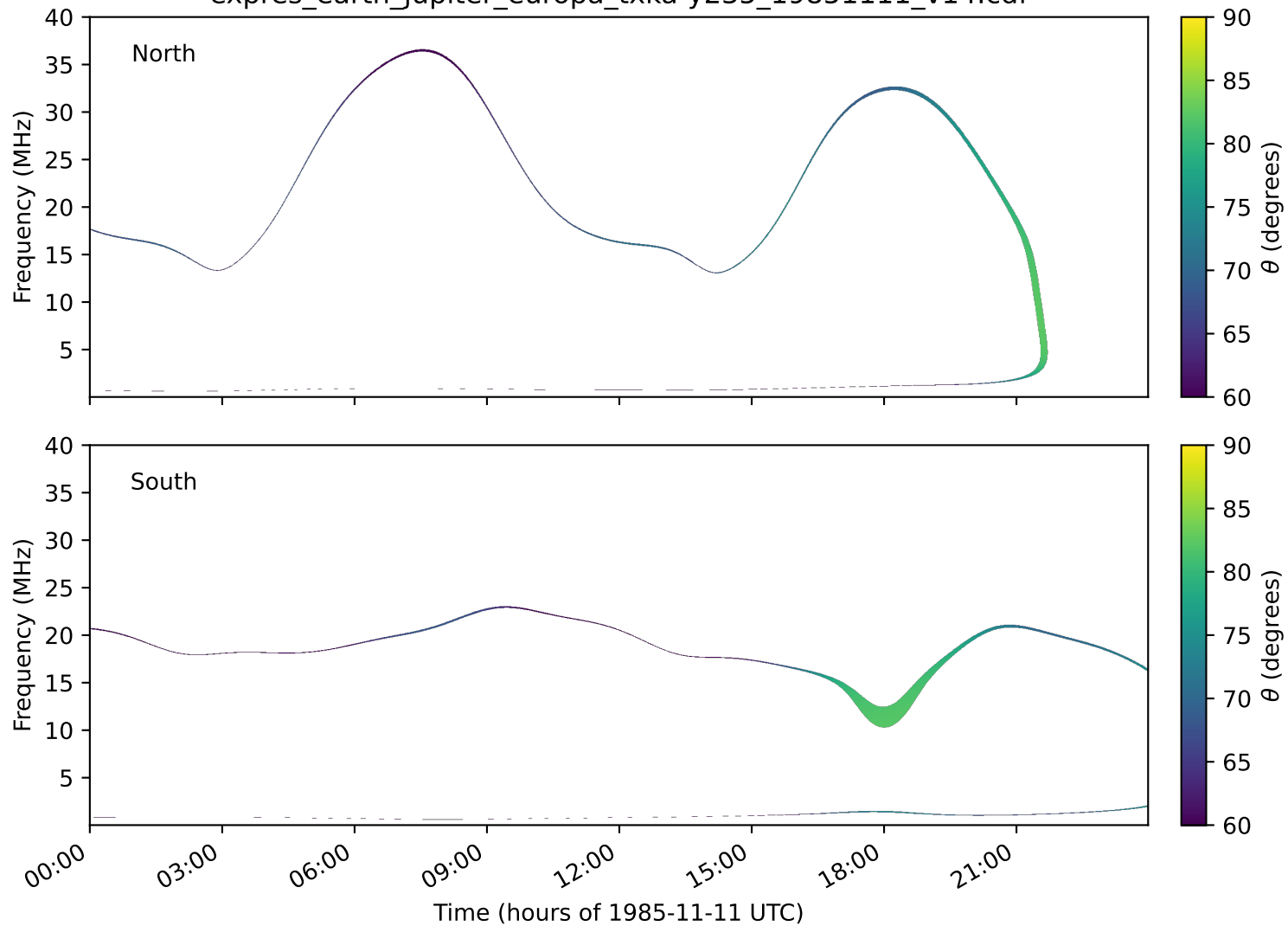
expres_earth_jupiter_europa_txka-y235_19851111_v14.cdf
