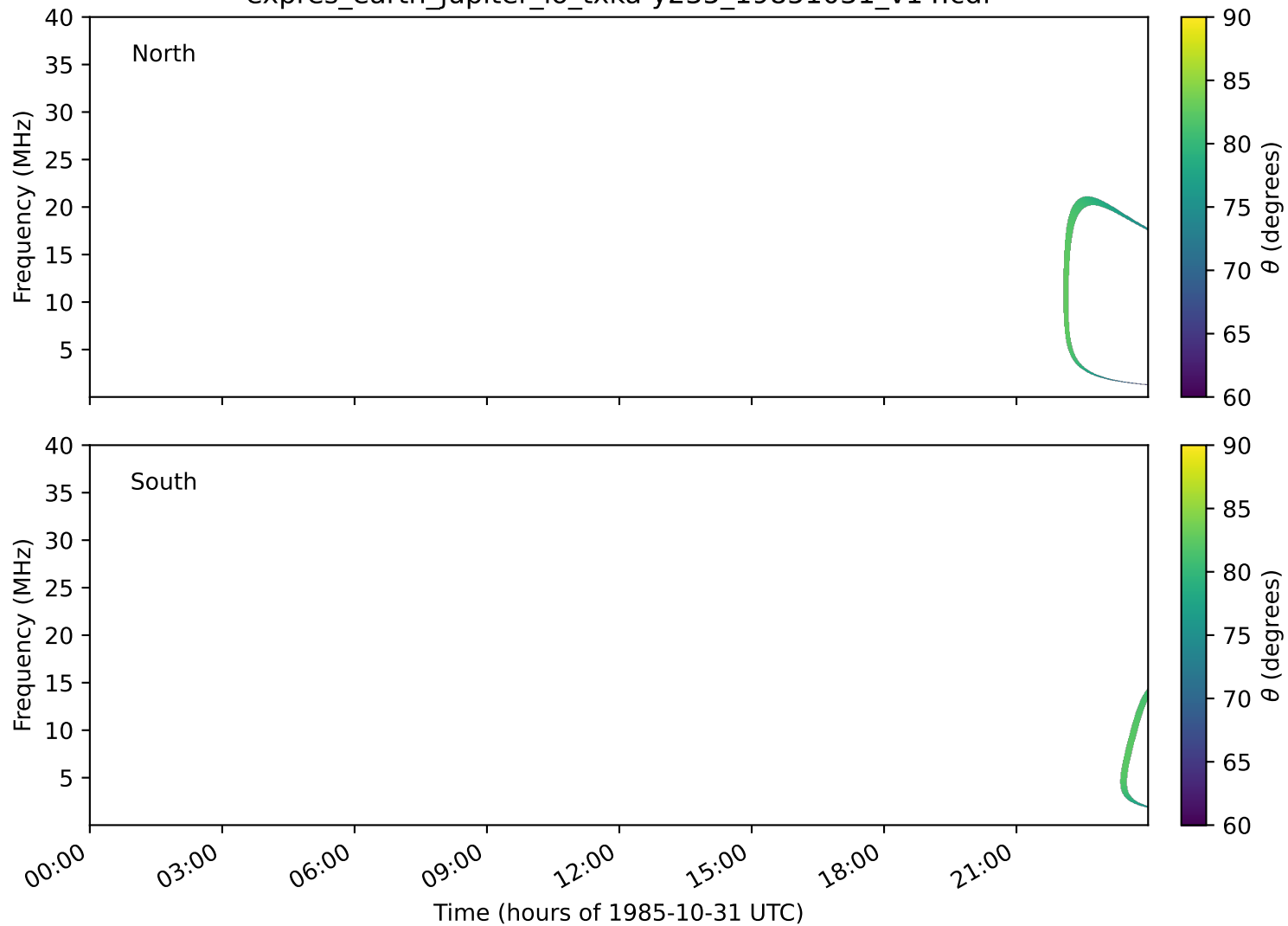
expres_earth_jupiter_io_txka-y235_19851031_v14.cdf
