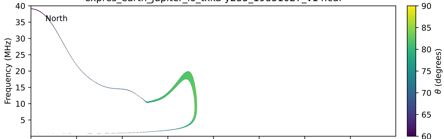
expres_earth_jupiter_io_txka-y235_19851027_v14.cdf
