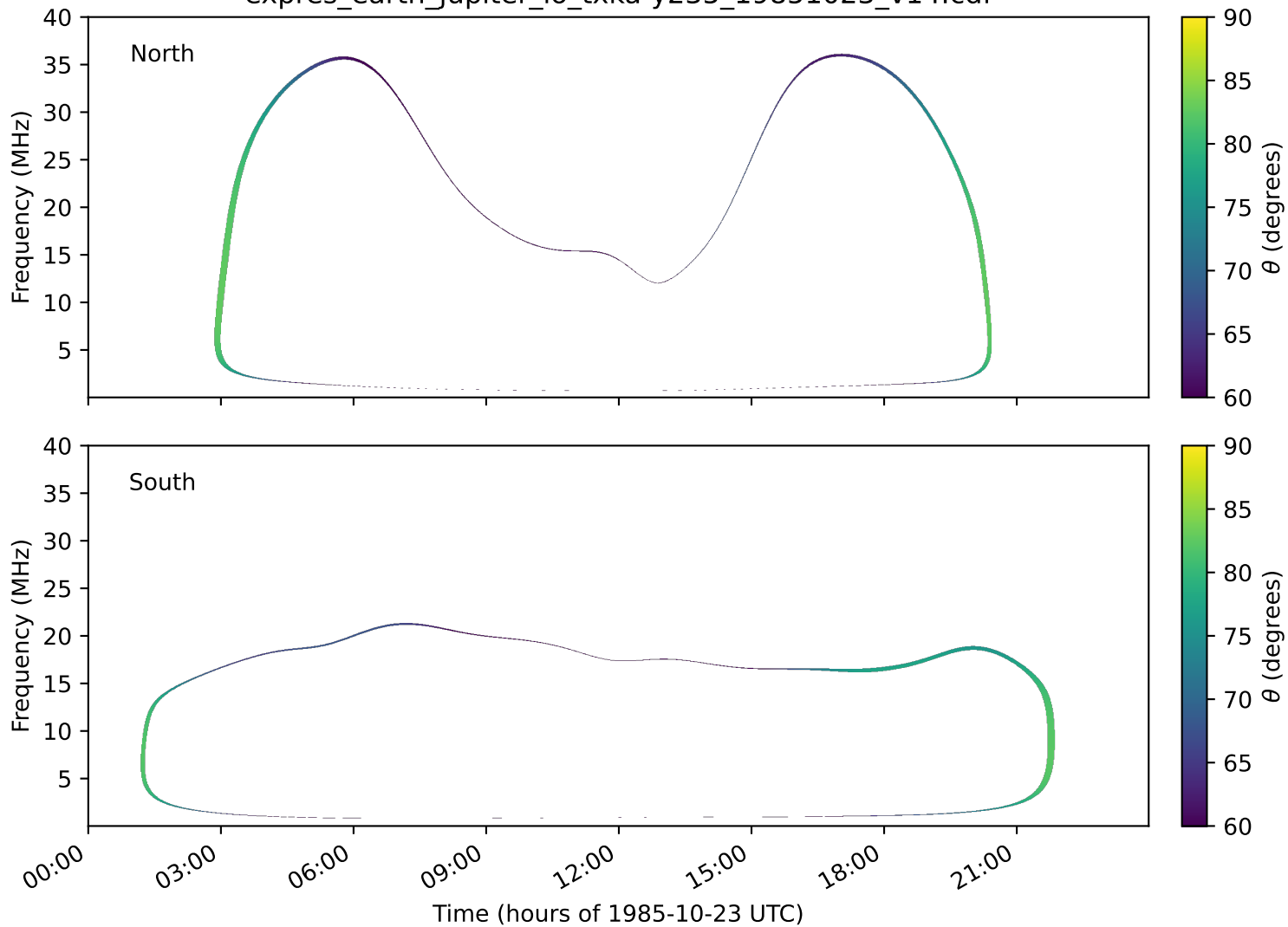
expres_earth_jupiter_io_txka-y235_19851023_v14.cdf
