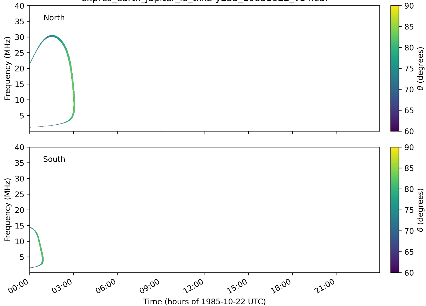
expres_earth_jupiter_io_txka-y235_19851022_v14.cdf
