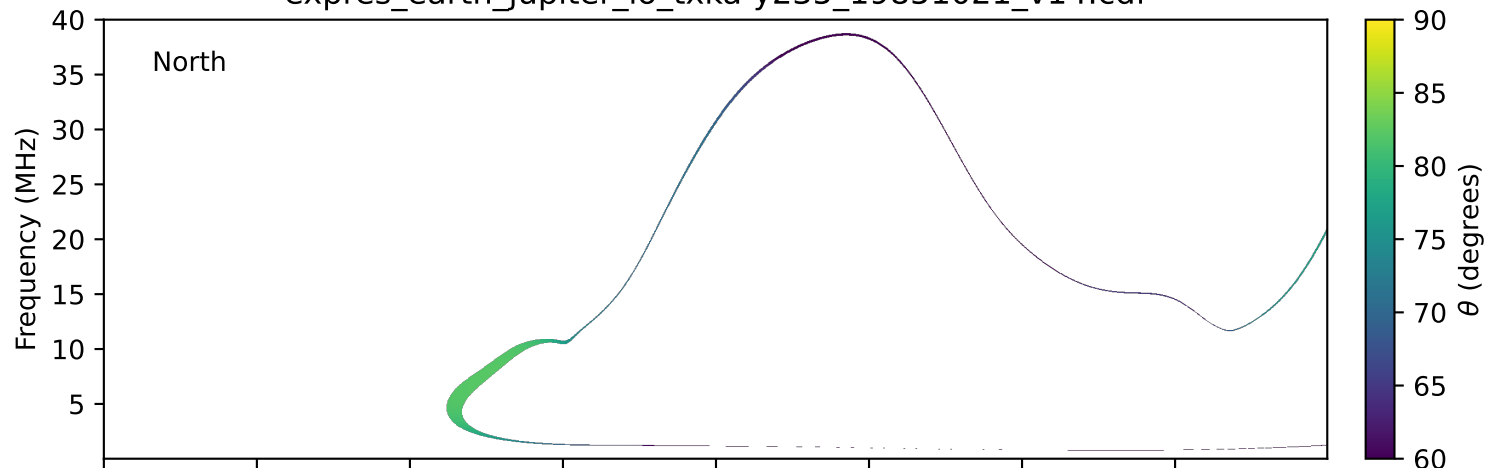
expres_earth_jupiter_io_txka-y235_19851021_v14.cdf
