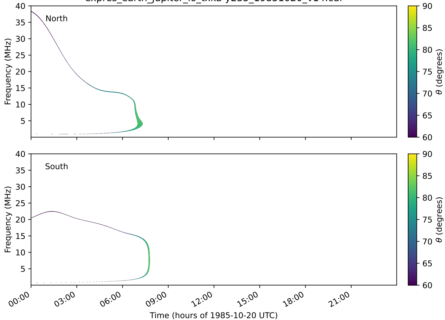
expres_earth_jupiter_io_txka-y235_19851020_v14.cdf
