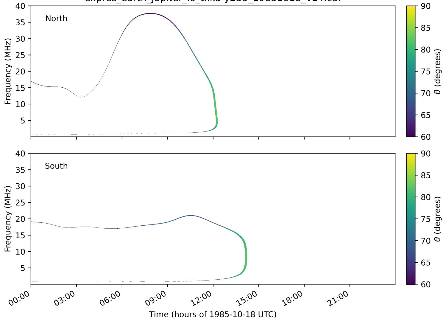
expres_earth_jupiter_io_txka-y235_19851018_v14.cdf
