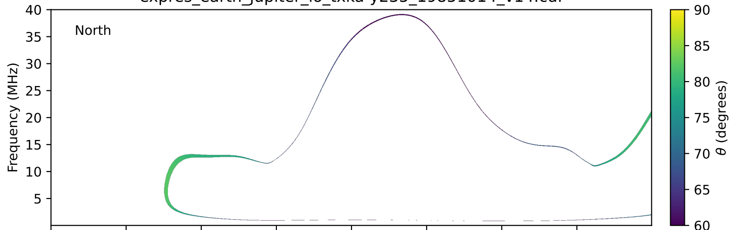
expres_earth_jupiter_io_txka-y235_19851014_v14.cdf
