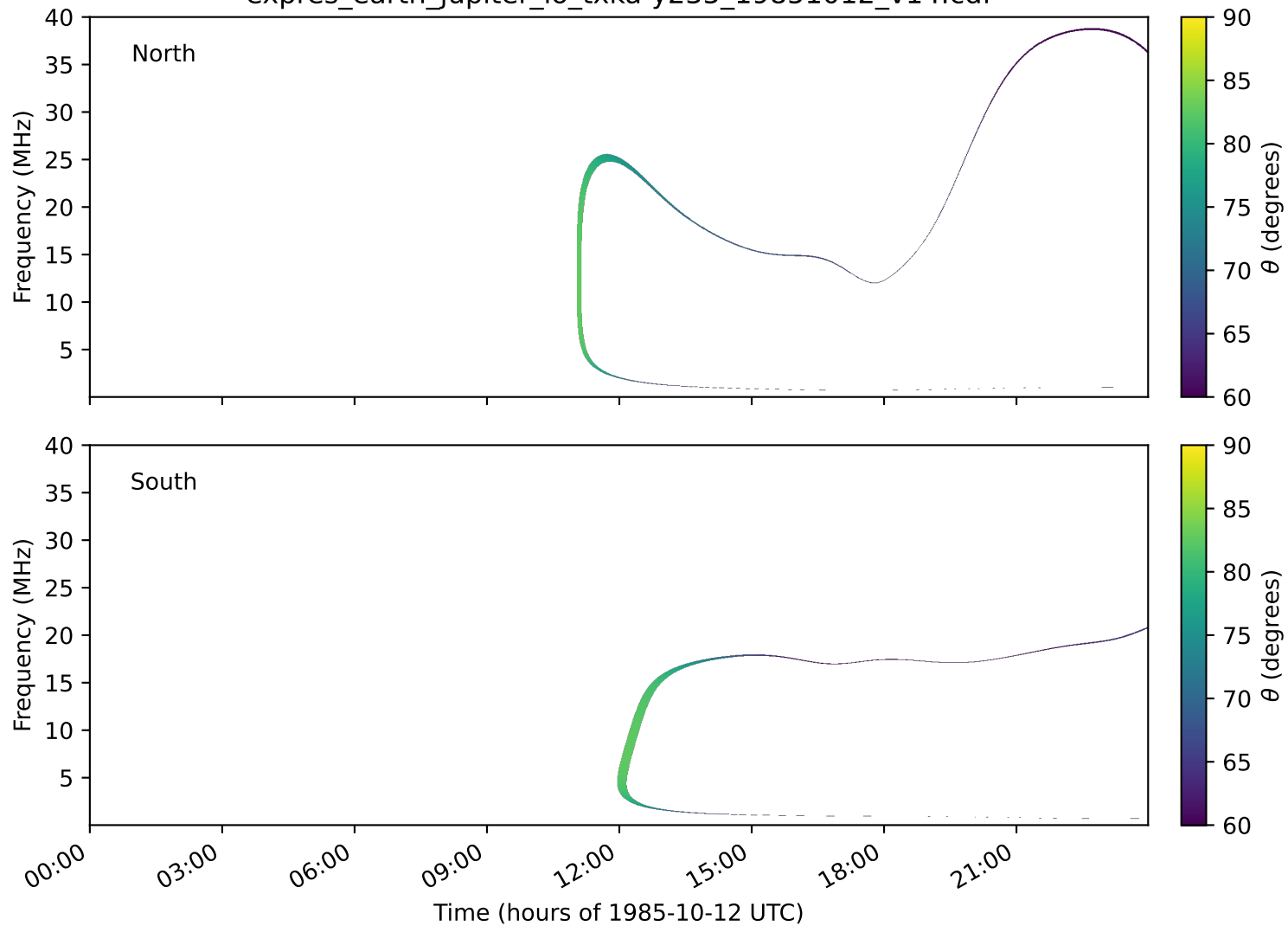
expres_earth_jupiter_io_txka-y235_19851012_v14.cdf
