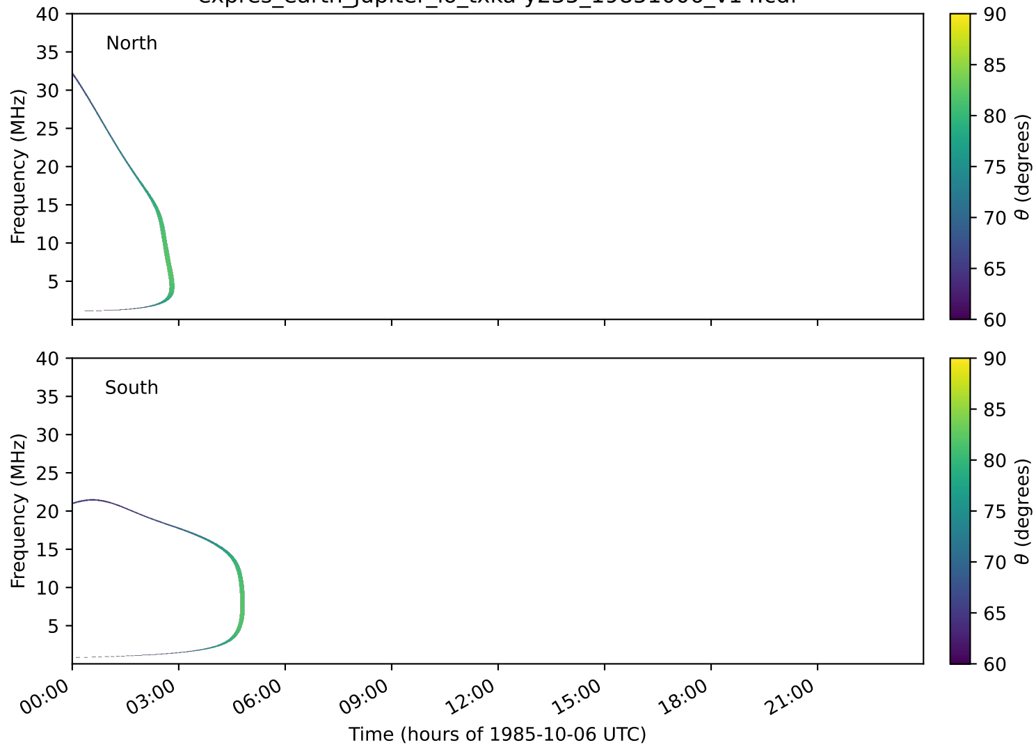
expres_earth_jupiter_io_txka-y235_19851006_v14.cdf
