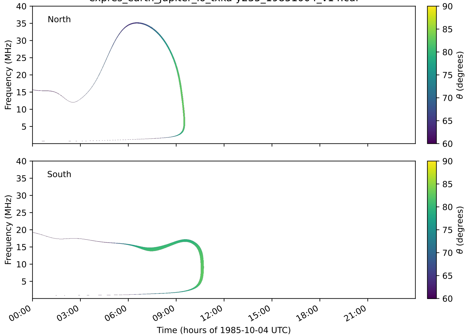
expres_earth_jupiter_io_txka-y235_19851004_v14.cdf
